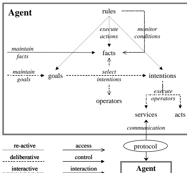
Figure 3. Behaviour Control Scheme pragmatic way without claiming to provide a base for rationality or intelligence in a human sense. Instead, the formal representation of declarative knowledge serves mainly as a common ground for interactions between agents providing a flexible and open scheme to express meaningful contents in a standardised and expressive way. On the other hand, the formal representation of procedural knowledge enables more autonomous, flexible, and explicit control of the behaviour of an agent. Combining both aspects, the formal descriptions of services enable reliable and dynamic interactions between agents.
