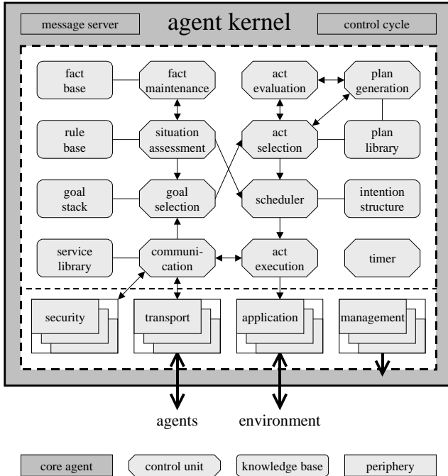
Figure 4. Roles of the Default Architecture. This architecture is still open for different implementations of the defined roles, but it is reasonable to implement default components for application-independent roles. Thus, an agent designer can compose a new agent reusing generic components and only needs to develop new components for application-specific tasks. Also, he can use only particular parts of the default architecture or even another control structure, as long as its interactive behaviour conforms to the requirements for service interactions (see Section 4.3).
