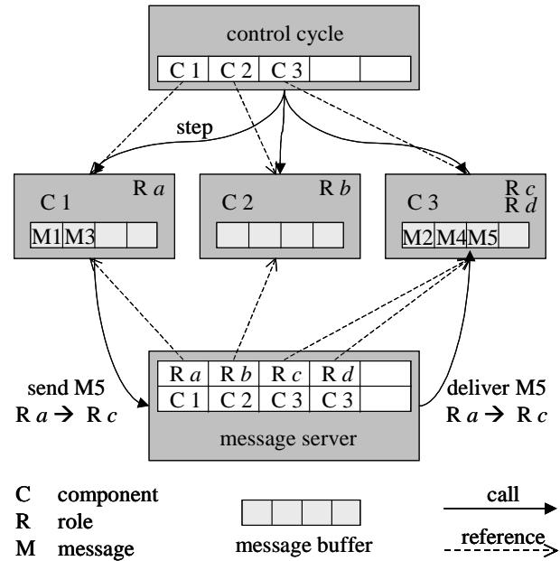
Figure 2. Interaction by Message Passing / Execution
